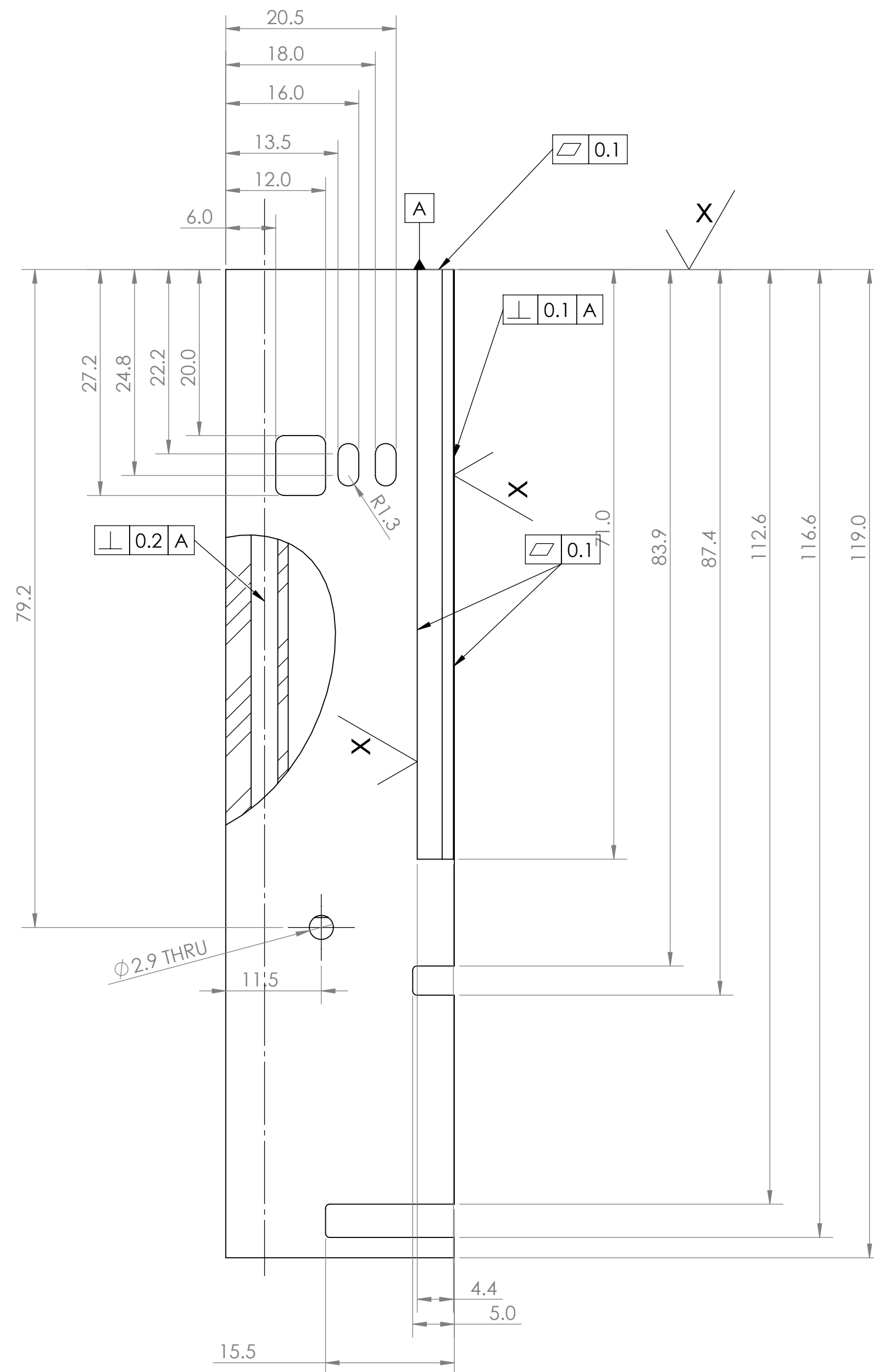
SECTION B-B
